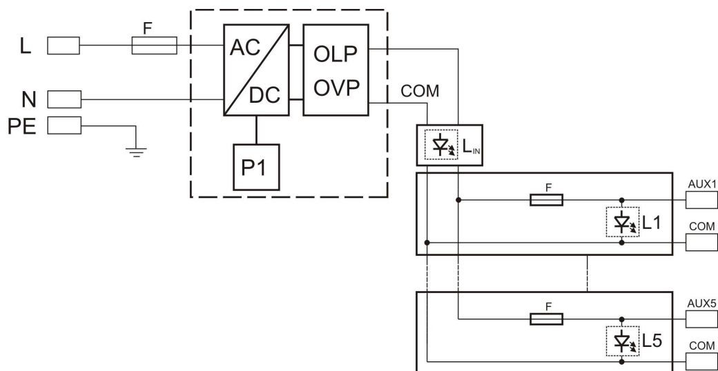
Fig.1. Block diagram of the PSU.
