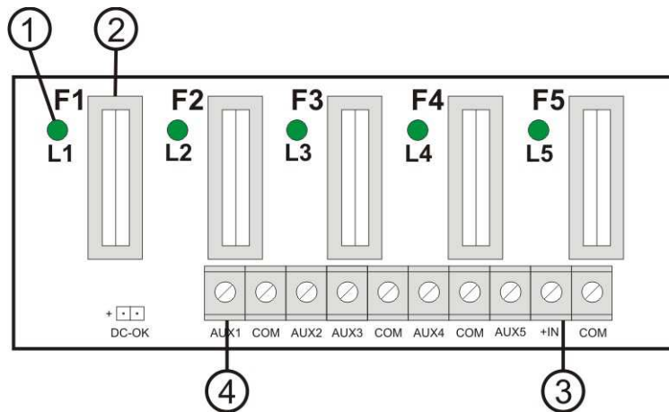
Fig.2. The view of the PSU's pcb.
