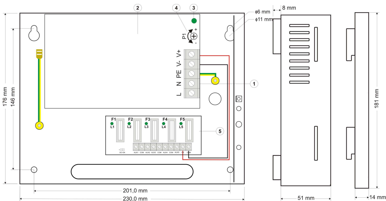
Fig.3. The view of the PSU.
