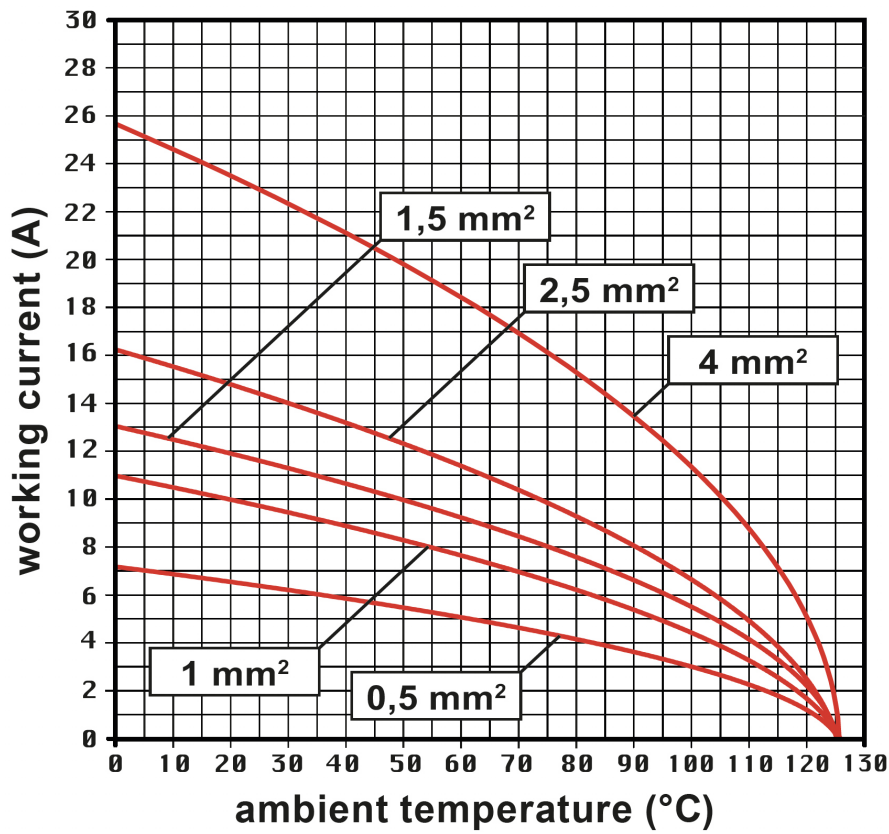
Derating curves
